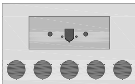
IC983002 20 in. Drop with Trailer Air, (1) 7-Way & (5) 4 in. Light Holes
