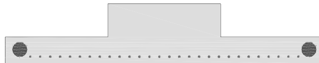
Reverse T-Bar with (2) 4 in. and (28) 3/4 in. Round Light Holes
