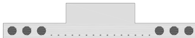
Reverse T-Bar with (6) 4 in. and (16) 3/4 in. Round Light Holes
